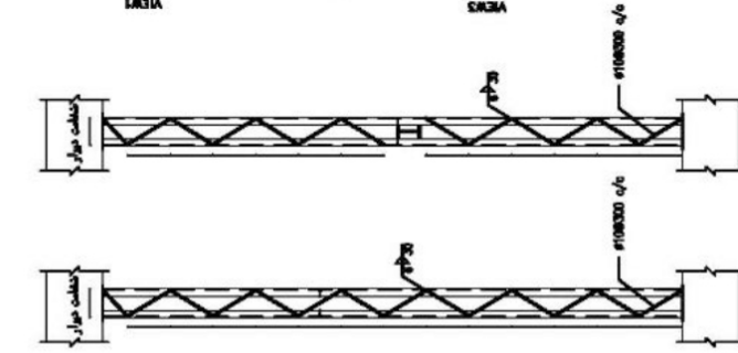
DETAIL-5 Sc. 1:10
